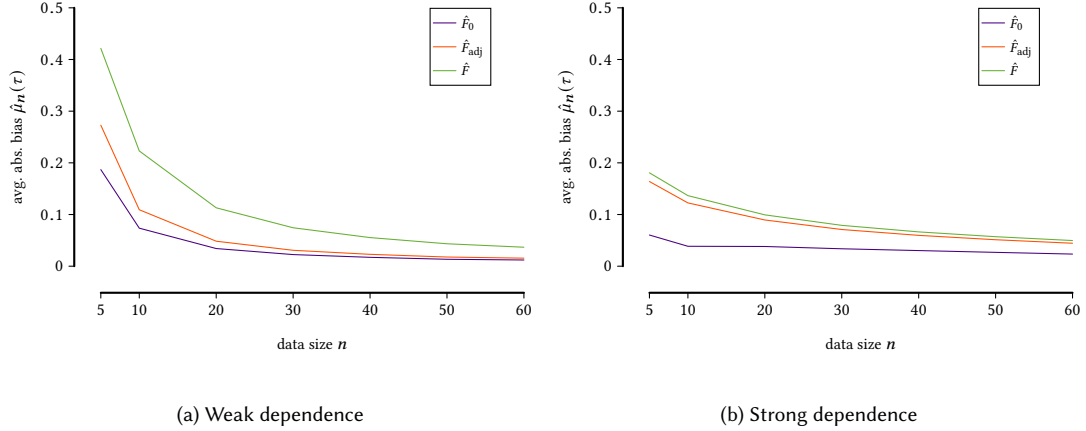
Fig. 3. Estimated absolute bias \hat{\mu}_n(\tau) of estimators \tau = \hat{F}, \hat{F}_{\text{adj}} , and the reliable fraction of information \hat{F}_0 , averaged over p \in P[0, 0.25] (left) and over p \in P[0.75, 1] (right), across different data sizes n .
