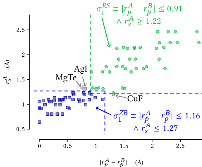
Fig. 7. Binary semiconductors that crystallize as zincblende (boxes) and rocksalt (circles); blue and green materials are correctly classified by subgroup-based prediction model—the involved rules (annotated) use elements of top functional dependency as two out of three variables. (source: Goldsmith et al. [8]).
